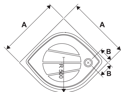
Elipso Pro 80 A = 800 mm Elipso Pro 90 A = 900 mm Elipso Pro 100 A = 1000 mm B = 200 mm
